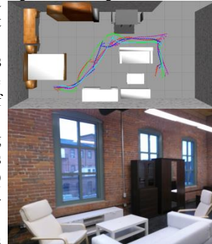
Fig 2: Wheelchair trajectories for 5 users from odometry, displayed in a 3D model (top) of the physical home environment tested (bottom). The odometry data for the other 5 users were corrupted and cannot be displayed.
